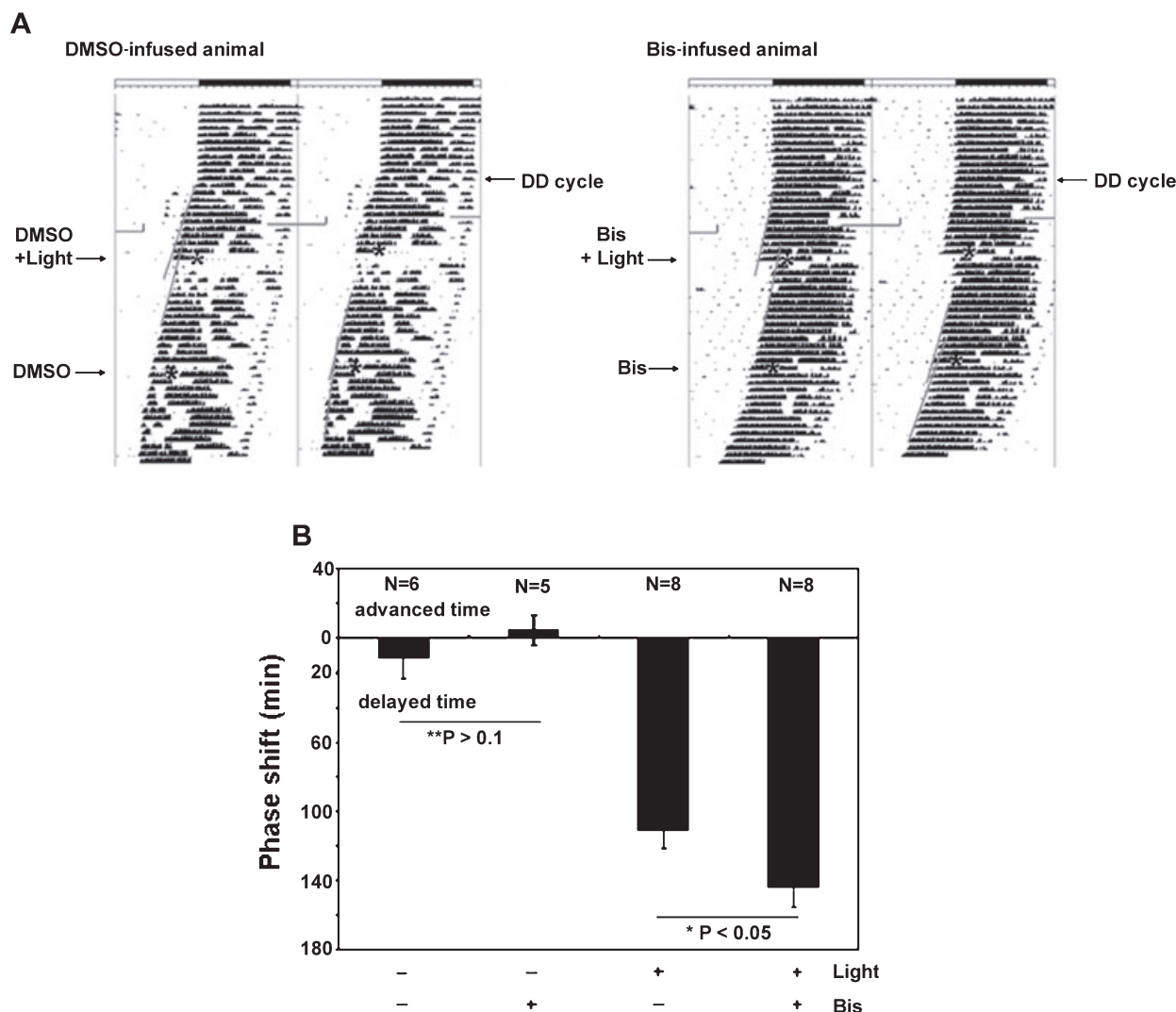
FIG. 3. Disruption of light-induced protein kinase C (PKC) activity augments the phase-shifting effect of light. (A) Representative double-plotted actographs. Initially, mice were maintained on a 12 h light/dark cycle, then dark adapted (DD). After 10 days of free running, mice were infused with either drug vehicle [dimethylsulfoxide (DMSO), left side] or the PKC inhibitor bisindolylmaleimide I (Bis) (right side) 30 min before light (50 lx, 10 min) exposure at circadian time (CT) 15 (*). Relative to the DMSO-infused animal, bisindolylmaleimide I administration enhanced the light-induced phase delay. To determine whether drug infusion altered timing in the absence of photic stimulation, mice were allowed to free run for an additional 14 days and then infused with DMSO or bisindolylmaleimide I at CT 14.5 (*). Regression lines approximate stimulus-induced phase shift. Please refer to Materials and methods for a description of the regression analysis. Horizontal bars in the activity record denote an 'off-line' period when wheel-running activity was not recorded. (B) Quantification of the phase-delaying effects of light. Mean \pm SEM of the phase-delaying effects of light. * P < 0.05 (significant), ** P > 0.1 (not significant), two-tailed Student's t -test. Numbers above bars denote sample size for each condition.
