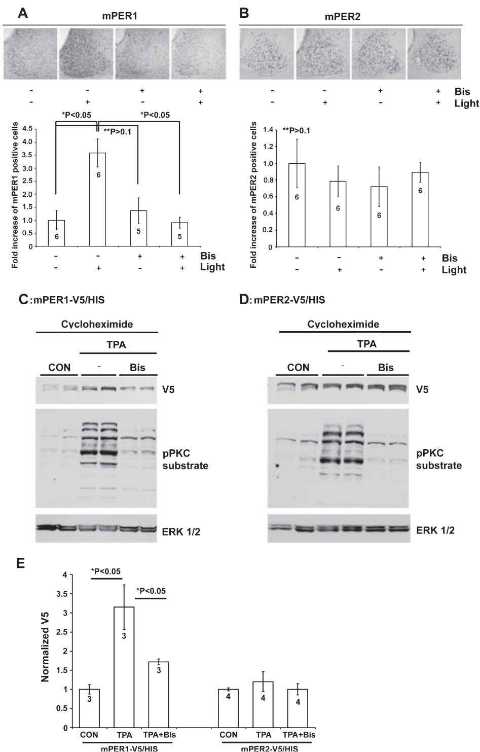
FIG. 5. Protein kinase C (PKC) regulates PER1 protein stability. (A and B) Mice were infused with drug vehicle (dimethylsulfoxide) or bisindolylmaleimide I (Bis) 30 min before light exposure (10 min, 100 lx) at circadian time 15. After light exposure, mice were returned to darkness for 90 min and then killed. Representative immunolabeling revealed that light triggered an increase in PER1 expression (A) that was attenuated by bisindolylmaleimide I. PER2 expression (B) was not affected by light. Quantification of PER1 and PER2 immunolabeling is shown below each data set. Error bars denote SEM. Numbers inside bars indicate the number of animals examined for each condition. For PER2, no significant difference was observed for any of the conditions ( P > 0.1 ). HEK 293T cells were transfected with mPER1-His-V5 (C) or mPER2-His-V5 (D) constructs. At 20 h after transfection, cells were pre-treated with cycloheximide (25 \mu\text{g}/\text{mL} , 60 min) and then stimulated with phorbol ester 12-O-tetradecanoylphorbol-13-acetate (TPA) (1 \mu\text{M} ). After 90 min of stimulation, cells were harvested and probed via western analysis. The V5 antibody was used to detect PER1 or PER2 fusion protein expression, PKC activity was assessed using the PKC substrate motif antibody and protein loading was examined using a total extracellular signal-regulated kinase (ERK) antibody. TPA administration led to an increase in PKC activity and PER1 stability. In contrast, TPA did not dramatically alter PER2 stability. Pre-treatment (30 min) with bisindolylmaleimide I (1 \mu\text{M} ) blocked TPA-induced PKC activity and reversed the stabilization of PER1. Representative samples were run in duplicate. These data indicate that PKC regulates PER1, but not PER2, stability. (E) Mean \pm SEM densitometric band analysis. Numbers inside bars indicate the number of experiments performed. Please refer to Materials and methods for a description of the western blotting quantification method. CON, control; pPKC, phospho-PKC. * P < 0.05 , ** P > 0.01 .
