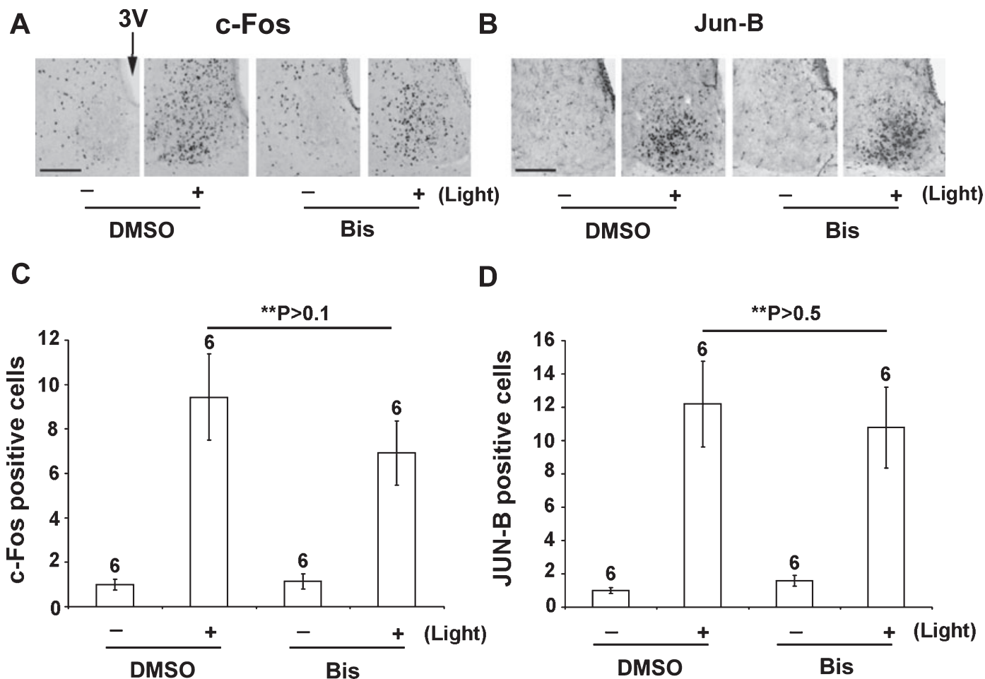
FIG. 4. Protein kinase C is not essential for light-induced light to immediate early gene expression in the suprachiasmatic nuclei. Drug vehicle [dimethylsulfoxide (DMSO)] or bisindolylmaleimide I (Bis) was infused 30 min before light exposure (10 min, 100 lx) at circadian time 15. After light exposure, mice were returned to darkness for 90 min and then killed. Immunolabeling revealed that light triggered robust c-Fos (A) and Jun-B (B) expression in mice infused with either DMSO or bisindolylmaleimide I. 3V, third ventricle. Bar, 125 \mu m. (C and D) Quantification of light-induced immediate early gene expression. Error bars denote SEM. Numbers above bars indicate the number of animals analysed for each condition. ** P > 0.1 (not significant). Arrow indicates 3V.
