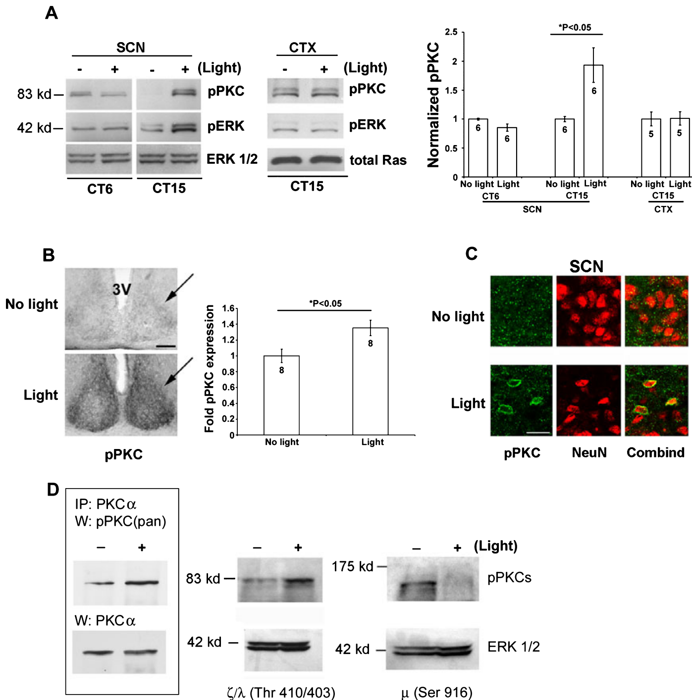
FIG. 1. Light-induced protein kinase C (PKC) phosphorylation in the suprachiasmatic nuclei (SCN). (A) Western analysis of SCN tissue from animals exposed to light (15 min, 100 lx) during the subjective night [circadian time (CT) 15] and subjective day (CT 6). Light exposure during the subjective night triggered an increase in the Ser 660 phosphorylated form of PKC (pPKC) in the SCN. Light also induced extracellular signal-regulated kinase (ERK)1 and ERK2 phosphorylation (pERK). In contrast, light did not induce PKC phosphorylation in the piriform cortex (CTX). As a protein-loading control, blots were stripped and probed for total ERK or Ras expression. Mean densitometric band analysis is shown to the right. Numbers inside bars indicate the number of experiments performed. Error bars denote SEM. (B) Immunohistochemical labeling detected a light-induced (CT 15, 15 min, 100 lx) increase in PKC phosphorylation in the SCN. Arrows denote approximate lateral SCN boundary. Bar, 125 \mu m. Quantification of pPKC-immunoreactive cells is shown to the right. Please refer to Materials and methods for a description of the quantification. Numbers within a bar denote the number of animals analysed. Error bars denote SEM. (C) SCN tissue from control (no light) and light-treated (15 min, 100 lux, CT15) animals was immunolabeled with antibodies against pPKC (green) and NeuN (red). A representative high-magnification image of the SCN shows the localized expression of pPKC and NeuN, indicating that light triggers PKC activity in neurons. Bar, 25 \mu m. (D) Light (15 min, 100 lux, CT15) regulation of PKC isozymes. (Boxed) SCN tissue was immunoprecipitated using a PKC \alpha antibody and probed using the phospho-Ser 660 PKC antibody. Light increased PKC \alpha phosphorylation relative to tissue from animals not exposed to light. Light triggered PKC \zeta/\lambda phosphorylation at Thr 410/403, respectively, in the SCN, whereas PKC \mu autophosphorylation at Ser 916 was decreased by photic stimulation. As a protein-loading control, blots were stripped and probed for total ERK levels. Data are representative of three independent experiments. For all western blotting, SCN were pooled from two animals for each experiment. 3V, third ventricle; IP, immunoprecipitate; W, western blot. * P < 0.05 .
