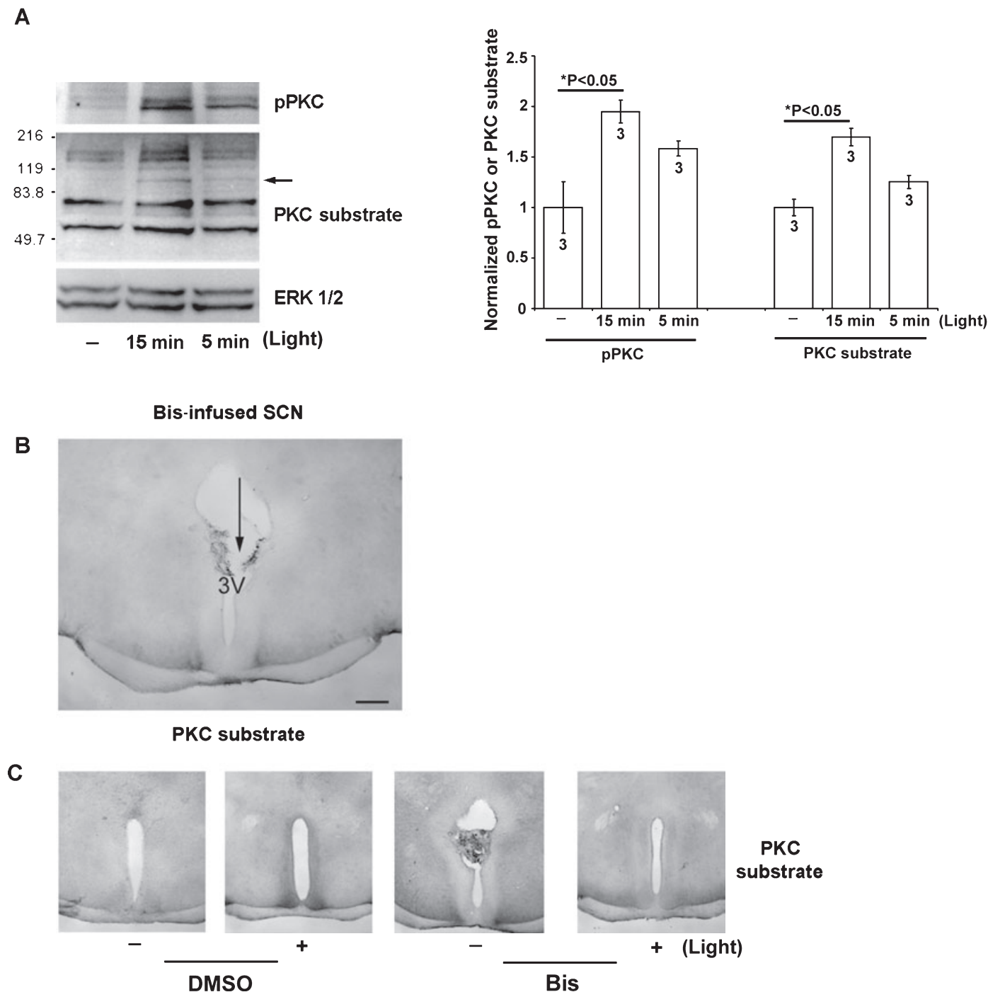
FIG. 2. Light-induced protein kinase C (PKC) activity in the suprachiasmatic nuclei (SCN). (A) SCN tissue from control mice (no light) and animals exposed to light (100 lx) were probed using a PKC phospho-substrate-specific antibody (PKC substrate). Relative to control animals, both 5 and 15 min of light triggered an increase in PKC substrate phosphorylation, indicating that light stimulates PKC enzymatic activity in the SCN. Paralleling this effect, levels of phospho-PKC (pPKC) increased with increasing light duration. As a protein loading control, the blot was also probed for total extracellular signal-regulated kinase (ERK) expression. Mean \pm SEM densitometric band analysis is shown to the left. For PKC substrate densitometric analysis, a representative band running at \sim 100 kDa (arrow) was analysed. Numbers inside bars indicate the number of experiments performed. Please refer to Materials and methods for a description of the quantification. (B) Disruption of PKC activity in the SCN. Cannulated mice were infused in the third ventricle with the PKC inhibitor bisindolylmaleimide I at circadian time (CT) 14.5. Mice were killed 30 min later and tissue was immunolabeled using the PKC phospho-substrate-specific antibody. This low-magnification representative image of the hypothalamus reveals the location of the infusion (arrow). 3V, third ventricle. Bar, 250 \mu m. (C) Cannulated mice were infused with dimethylsulfoxide (DMSO) (vehicle) or bisindolylmaleimide I (Bis) 30 min before light (15 min, 100 lx) exposure at CT 15. Coronal tissue sections were immunolabeled with the PKC phospho-substrate-specific antibody. Light triggered an increase in PKC substrate phosphorylation in animals infused with drug vehicle. In contrast, the infusion of bisindolylmaleimide I effectively blocked PKC enzymatic activity. *P < 0.05 .
